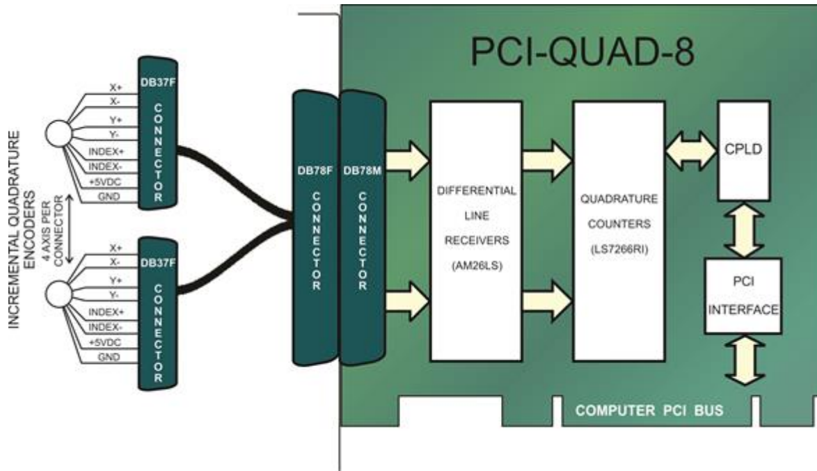
BLOCK DIAGRAM
